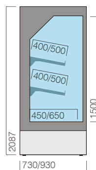
MF2 700 / 900 P CC FRUT 3M2 murais multi deck +3°... +6° C
