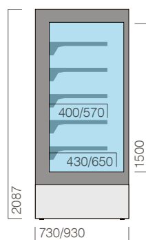
MF2 700 / 900P CC 3M1 murais multi deck +2°... +5° C
