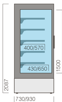
MF2 700 / 900P CP 3M1 murais multi deck 0°... +4° C
