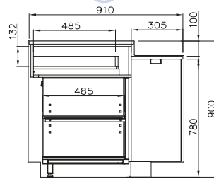
VMINPMR B caixa PMR PMR support counter caisse PMR caja PMR
