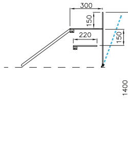
VMINPMR P caixa PMR PMR support counter caisse PMR caja PMR
