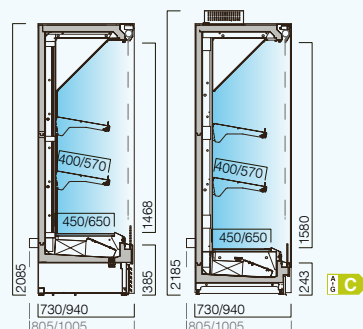
MF2 700/900 PF CC - CG 3H1 (+1...+10 °C)
